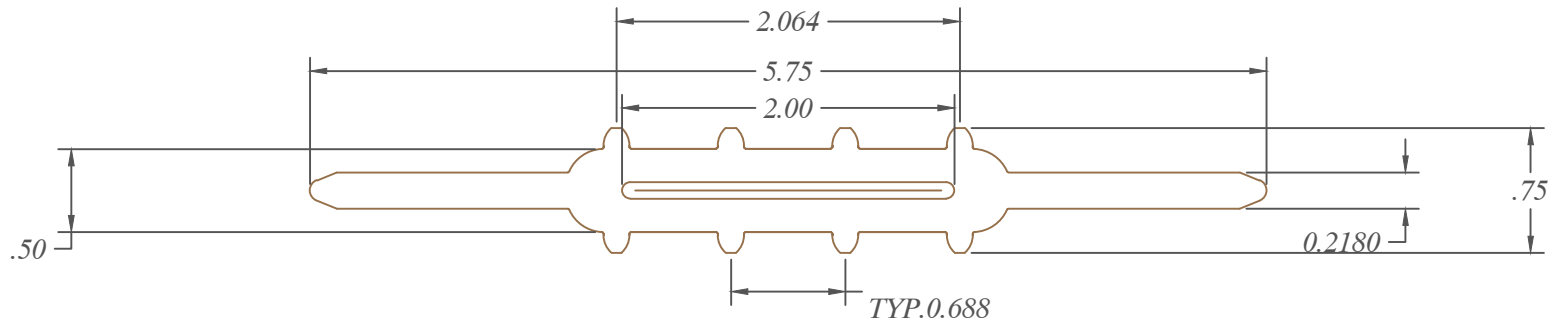
1 Inch Embedded flat fastener Part no:03-FL01
