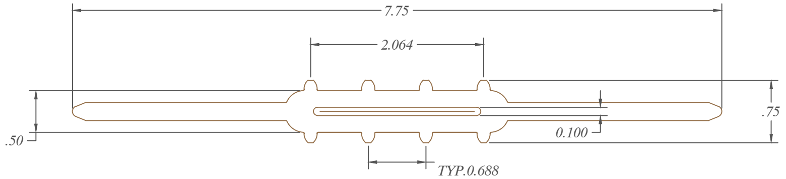
2 Inch Embedded flat fastener Part no:04-FL02
