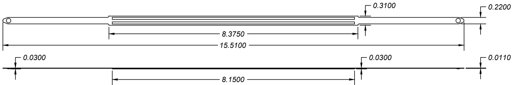
8 1/2 Base Part no:06-8B
